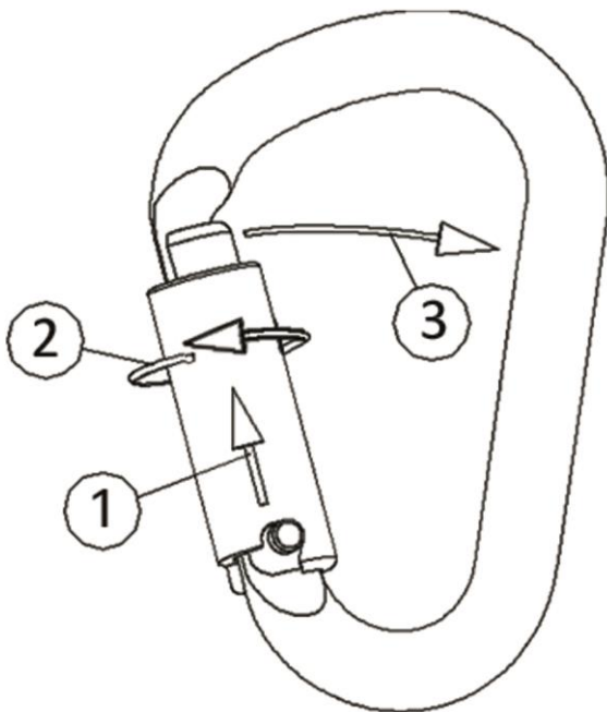
HMS SAFE-LOCK Carabiner: schematic figure
